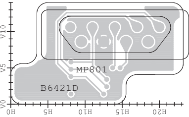
• JACK UNIT (TOP VIEW)
