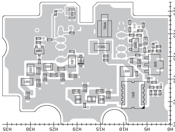
• VR UNIT (BOTTOM VIEW)
