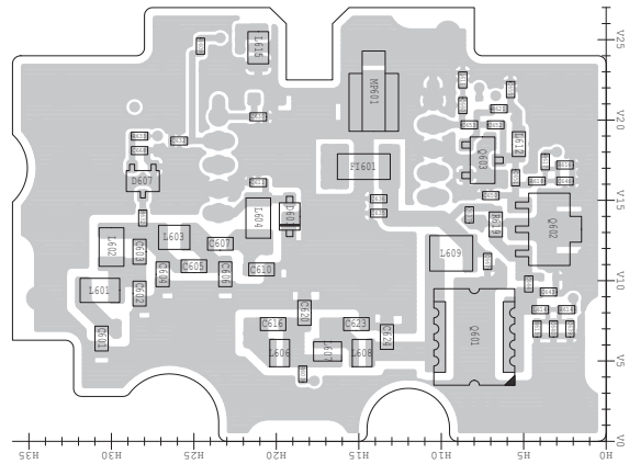
• VR UNIT (BOTTOM VIEW)
