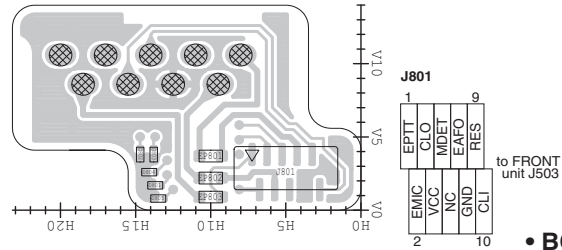
• JACK UNIT (BOTTOM VIEW)
