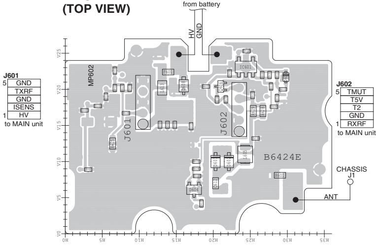
• VR UNIT (TOP VIEW)
